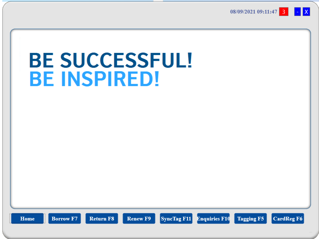
Fig. 2 Middleware Homepage
